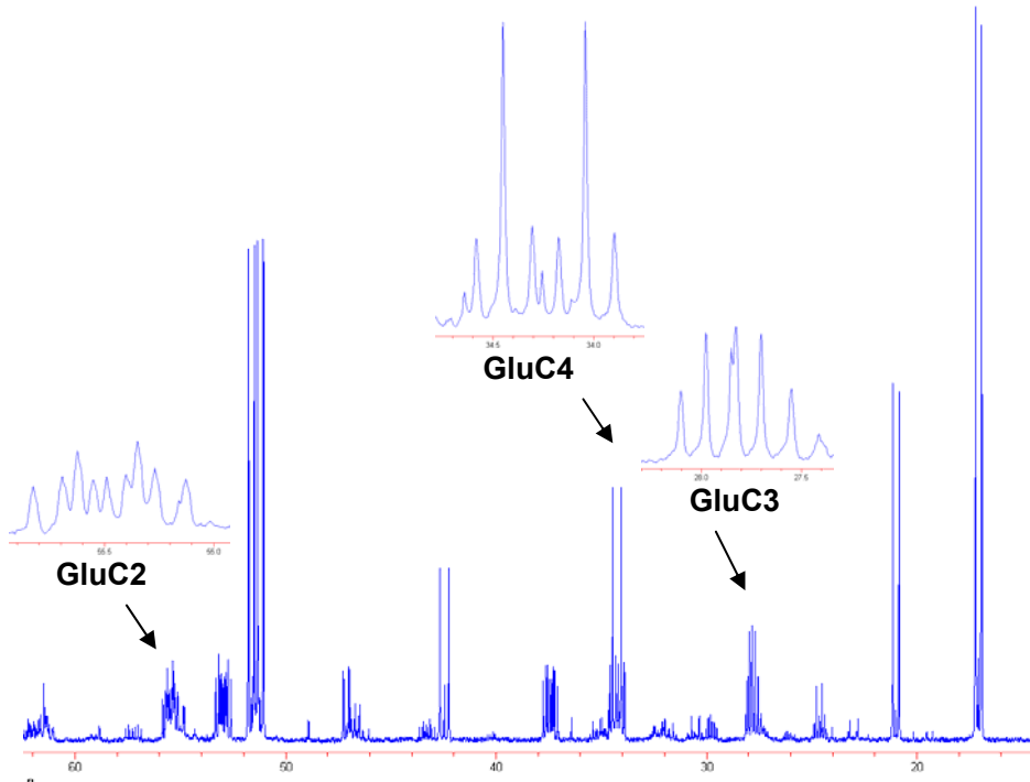
Figure 4.6 Representative ^{13}\text{C} NMR spectrum obtained after ^{13}\text{C} labeling and extraction of 7 ml of Frozen beads incubated in basal medium for 1 hour followed by labeling medium for 6 hours.
