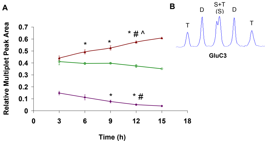
Figure 4.3 A). Relative multiplet peak areas of the glutamate C3 (GluC3) resonance during incubation in 15 mM U- 13 Cglucose DMEM for 3-15 hours. The singlet (S) multiplet is represented by the purple line, doublet (D) by the green line, and the triplet (T) by the red line. B). Representative glutamate C3 resonance with multiplets labeled. * p < 0.05 compared to 3 hour time point, # p < 0.05 compared to 6 hour time point, ^ p < 0.05 compared to 9 hour time point. n = 3 for 3-12 hour incubations and n = 1 for 15 hour incubation.
