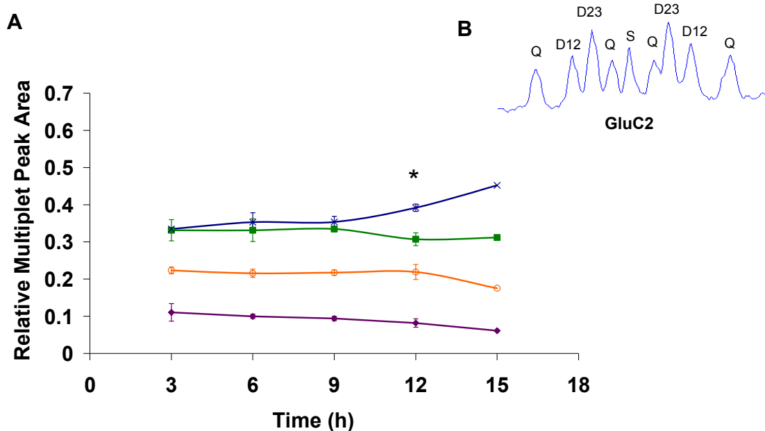
Figure 4.2 A). Relative multiplet peak areas of the glutamate C2 (GluC2) resonance during incubation in 15 mM U- 13 Cglucose DMEM for 3-15 hours. The quartet (Q) multiplet is represented by the blue line, doublet 23 (D23) by the green line, doublet 12 (D12) by the orange line, and the singlet (S) by the purple line. B). Representative glutamate C2 resonance with multiplets labeled. *indicates p < 0.05 compared to 3 hour time point. n = 3 for 3-12 hours and n = 1 for 15 hours.
