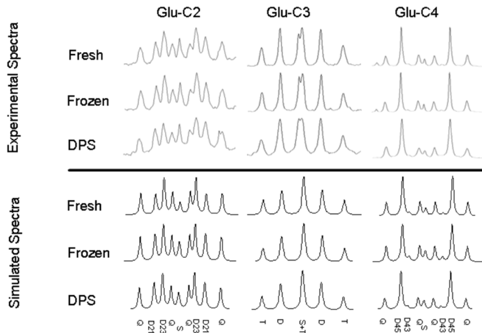
Figure 5.3 Representative isotopomer patterns from glutamate C2, C3, and C4 resonances from experimental spectra obtained from extracts of Fresh, Frozen, and DPS-vitrified encapsulated \beta TC-tet cells and simulated spectra obtained from tcaSIM based on tcaCALC output. A modified single pyruvate pool model was used to determine the tcaCALC output. The different multiplet components are represented by Q (quartet), D (doublet), S (singlet), and T (triplet).
