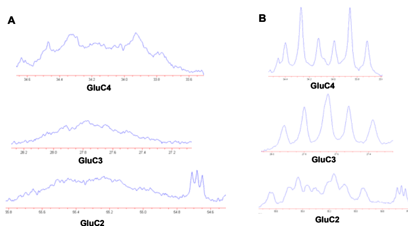
Figure B.1 Glutamate resonances from ^{13}\text{C} NMR spectra obtained from extractions using A). metal generator probe and B). a plastic Omin Tip™ generator probe. Prior to each extraction, a 6 ml bead volume of Fresh beads was incubated in 0 mM glucose DMEM for 1 hour followed by 12 hour incubation in ^{13}\text{C} -glucose medium.
