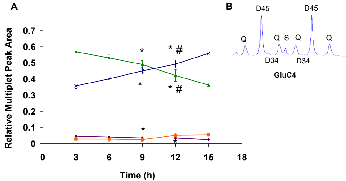
Figure 4.4 A). Relative multiplet peak areas of the glutamate C4 (GluC4) resonance during incubation in 15 mM U- 13 Cglucose DMEM for 3-15 hours. The singlet (S) multiplet is represented by the purple line, doublet 45 (D45) by the green line, quartet (Q) by the blue line, and doublet 34 (D34) by the orange line. B). Representative GluC4 resonance with multiplets labeled. * p <0.05 compared to the 3 hour time point, # p <0.05 compared to 6 hour time point. n =3 for 3-12 hour incubations and n =1 for 15 hour incubation
