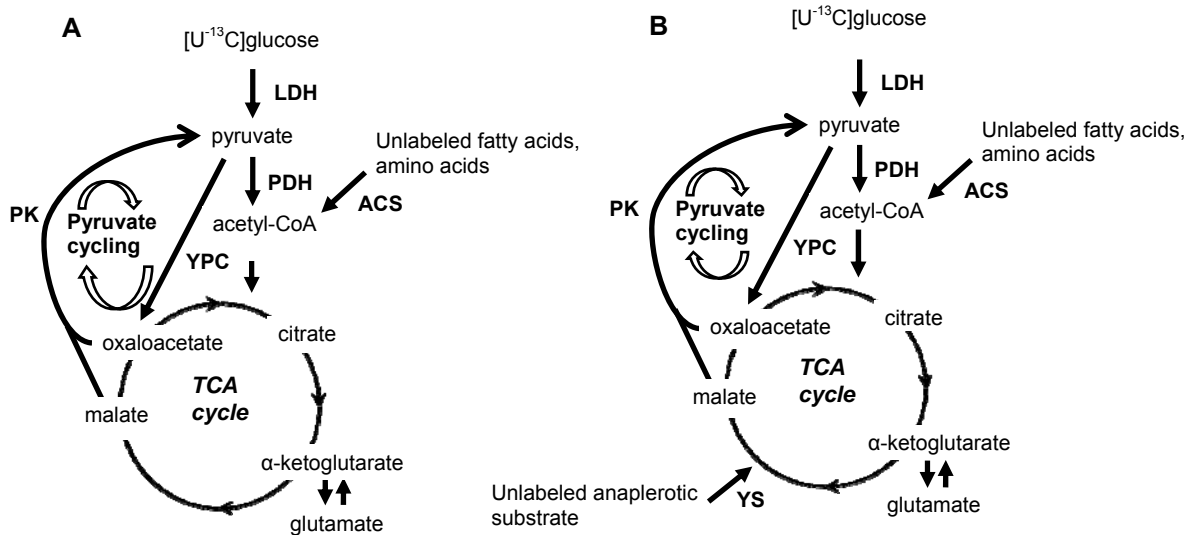
Figure 4.8 A). Standard model and B). a previously published modified model of glucose metabolism containing a second non-pyruvate carboxylase entrance to the TCA cycle applied in tcaCALC [36]. Adapted from Simpson et al [36]. The tcaCALC fluxes represented above are PK (phosphoenol-pyruvate carboxykinase/pyruvate kinase or malic enzyme); LDH (glycolysis); PDH (pyruvate dehydrogenase); YPC (pyruvate carboxylase); ACS (acetyl-CoA synthetase); and YS (non-pyruvate carboxylase anaplerosis).
