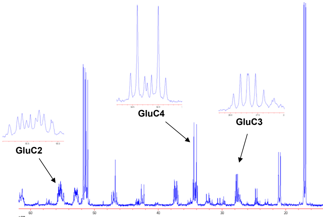
Figure 4.7 Representative ^{13}\text{C} NMR spectrum obtained after ^{13}\text{C} labeling and extraction of 12 ml of DPS-vitrified beads incubated in basal medium for 1 hour followed by labeling medium for 6 hours.
