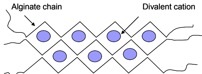
Figure 3.1 The “egg box model.” Adapted from Grant et al. [89]
