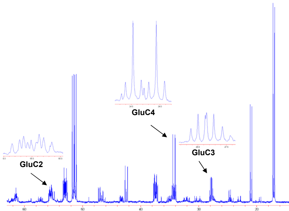
Figure 4.1 Representative ^{13}\text{C} NMR spectrum obtained after ^{13}\text{C} labeling and extraction on 6 ml of Fresh beads incubated in labeling medium for 6 hours.
