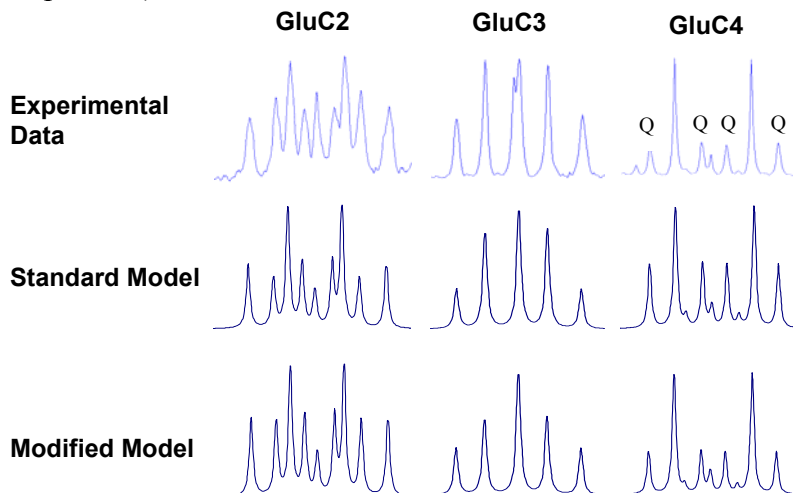
Figure 4.8 A). Standard model and B). a previously published modified model of glucose metabolism containing a second non-pyruvate carboxylase entrance to the TCA cycle applied in tcaCALC [36]. Adapted from Simpson et al [36]. The tcaCALC fluxes represented above are PK (phosphoenol-pyruvate carboxykinase/pyruvate kinase or malic enzyme); LDH (glycolysis); PDH (pyruvate dehydrogenase); YPC (pyruvate carboxylase); ACS (acetyl-CoA synthetase); and YS (non-pyruvate carboxylase anaplerosis).
