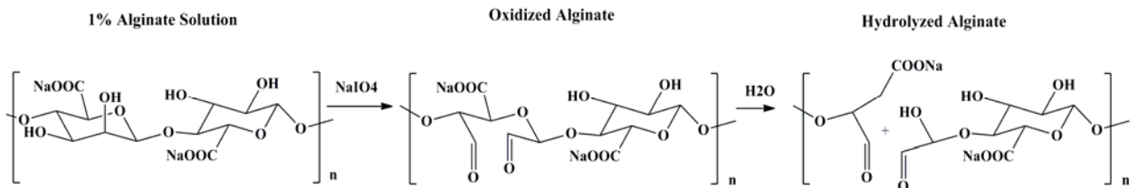
Figure 3.3 Sodium periodate oxidation of alginate. Figure adapted from [111]. During the oxidation procedure, the cis -diol group on the uronate residue is cleaved to form an open-chain adduct. The resulting alginate is susceptible to hydrolysis.
