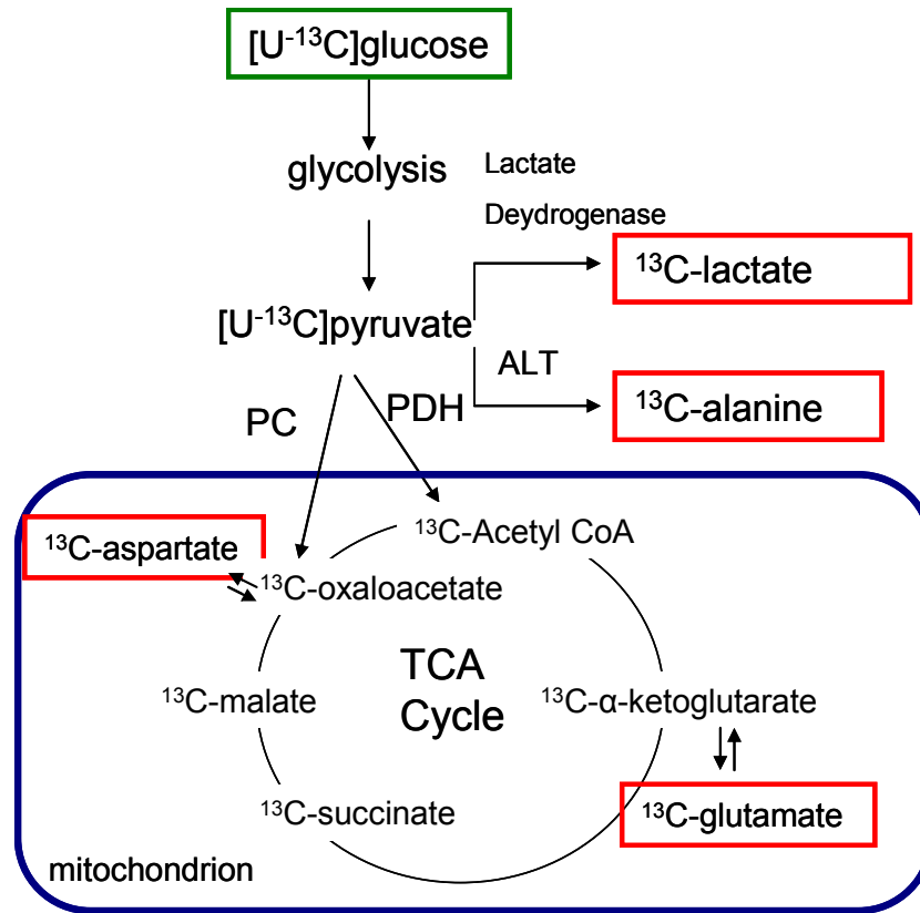
Figure 3.4 Labeling of metabolites in the cell after introduction of U- 13 C (uniformly labeled- 13 C) glucose. Metabolites in red have high enough intracellular concentrations to be detected by NMR. PC (pyruvate carboxylase); PDH (pyruvate dehydrogenase); ALT (alanine aminotransferase) (Adapted from Papas et al.[180]).
