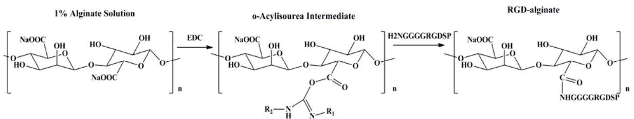
Figure 3.2 RGD conjugation to alginate via carbodiimide chemistry. Adapted from [98, 108]. The 1-Ethyl-3-[3-dimethylaminopropyl] carbodiimide hydrochloride (EDC) forms an O-acylisourea intermediate which is stabilized by N -hydroxysulfosuccinimide (sulfo-NHS). An amide bond is then formed between the N-terminal amine on the RGD peptide and the carboxyl group on the alginate chain.
