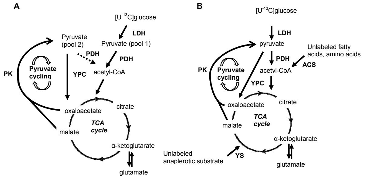
Figure 3.5 Two models of mitochondrial metabolism in the beta cell that have been applied in the tcaCALC modeling program to calculate metabolic fluxes, adapted from Simpson et al. [36]. A).a dual pyruvate pool model, B). a modified single pool model with a second non-pyruvate carboxylase anaplerotic substrate entrance to the TCA cycle.
